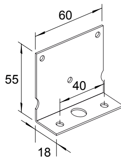
L-shaped metal mounting bracket 6401
