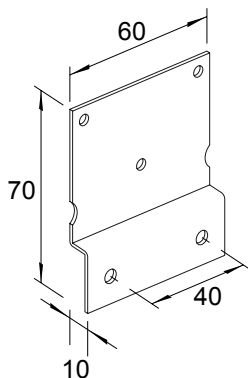
S-shaped metal mounting bracket 6402
