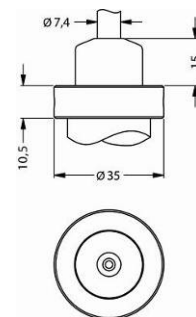
cable outlet, cable with ventilation tube (IP 68) 8
